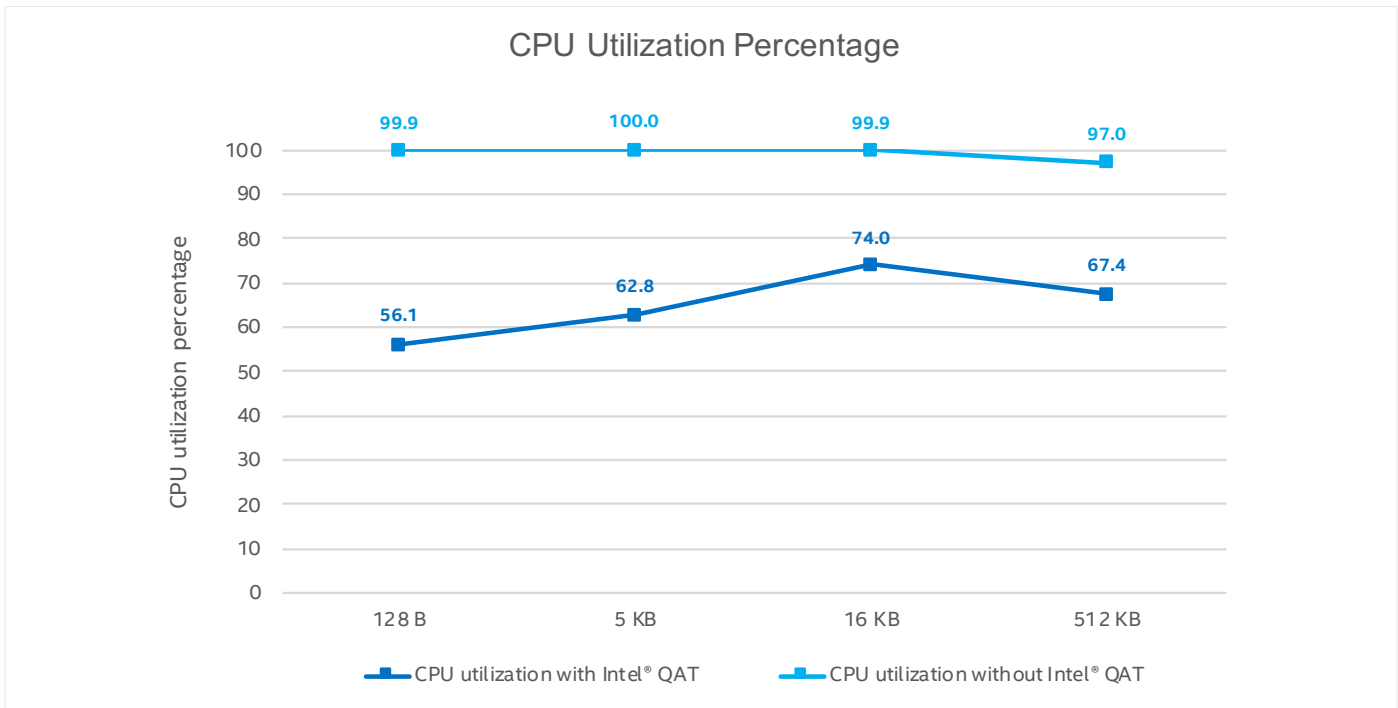
Figure 3. CPU utilization for encryption functionality with Intel® QAT and without. 1
