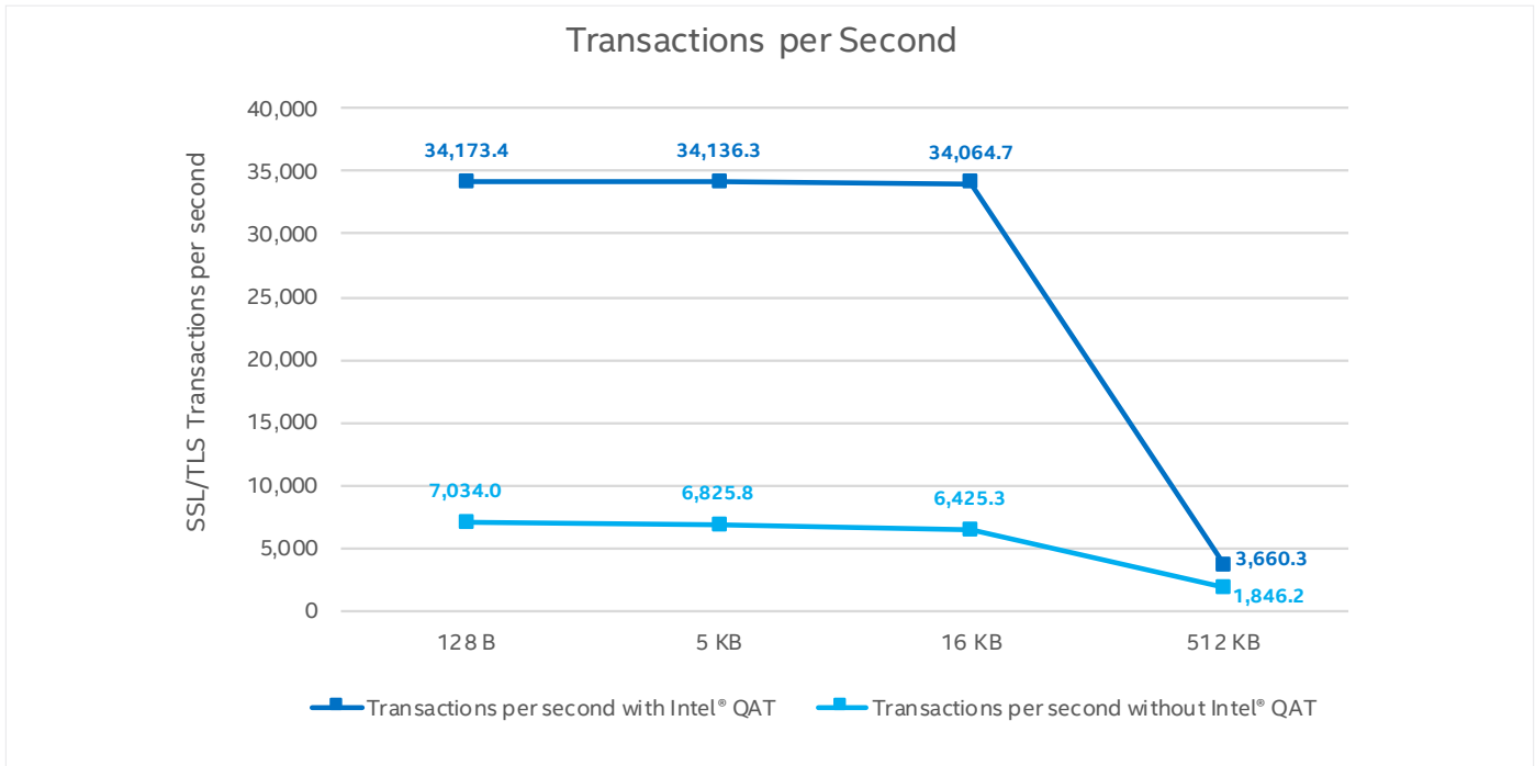
Figure 2. SSL/TLS transactions per second with Intel® QAT and without. 1
