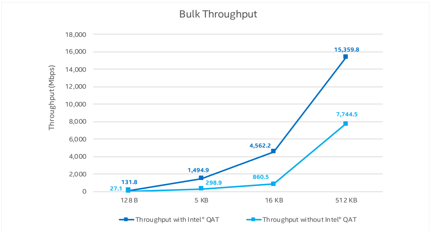
Figure 1. Bulk throughput with Intel® QAT and without. 1
